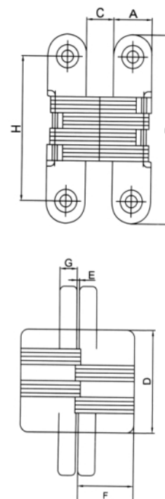
(暗铰链外形尺寸图)
