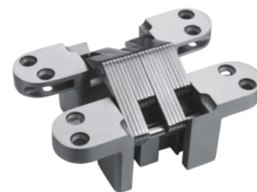
型号: HCG001 尺寸: 34X140X28mm
