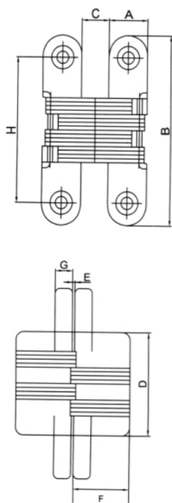
(暗铰链外形尺寸图)
