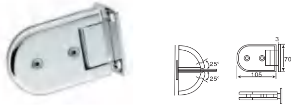
GC-046 半圆长形135° 浴室玻璃夹 A long 135 degree bathroom glass clamp
