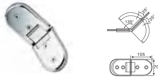
GC-046 半圆长形135° 浴室玻璃夹 A long 135 degree bathroom glass clamp
