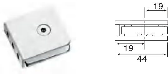
GC-001 方形固定夹0° Square fixing clip 0°
